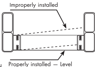
FIGURE 2 CROSSOVER DRAINAGE
